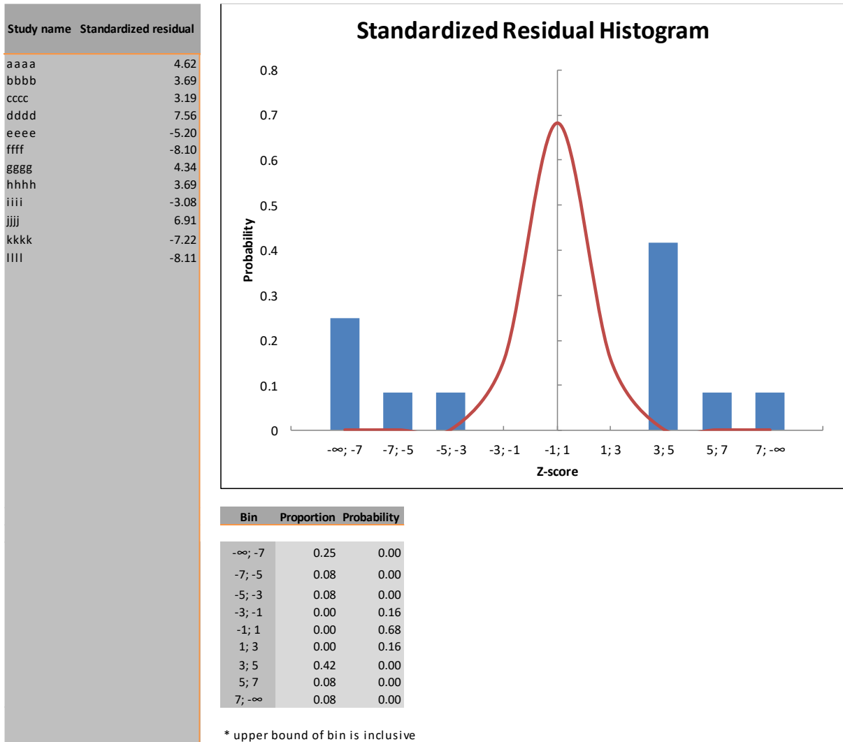
Figure 23: Example of Standardized Residual Histogram part
